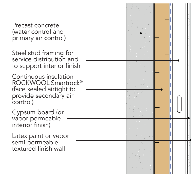
Figure 5: ROCKWOOL Smartrock® insulation controls internal air convection; continuity of the secondary air control layer is achieved by taping and sealing the facer joints, seams, terminations, and penetrations.
